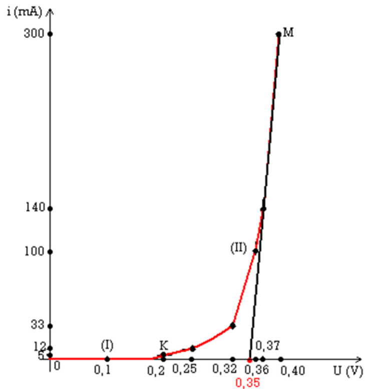
Figure 13.9 : Graphe I = f(U)
