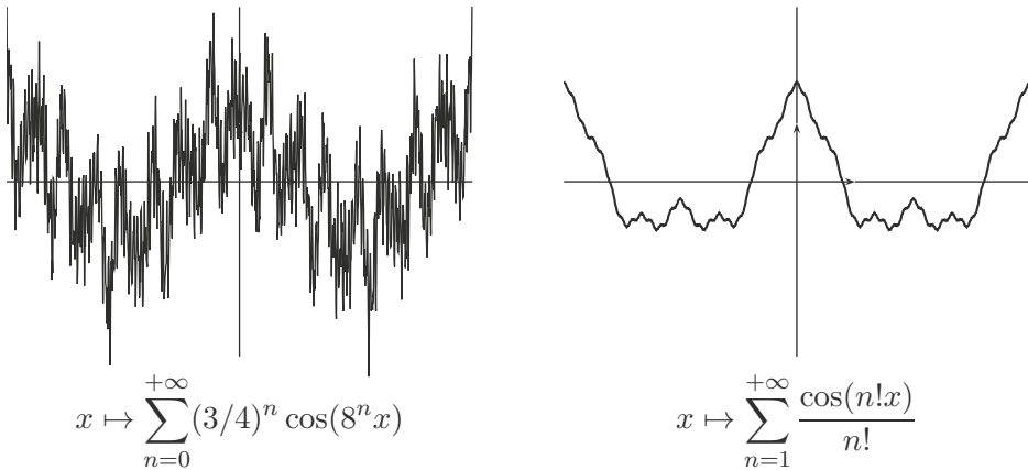
FIGURE II.4.5 – Fonctions continues mais nulle part dérivable
