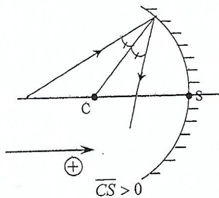
miroir concave
