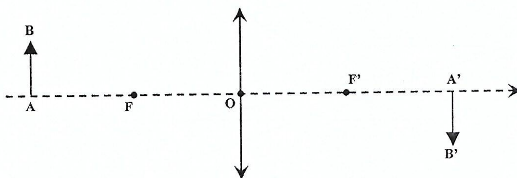
Figure 14 : Lentille mince
