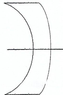
Ménisque divergent
