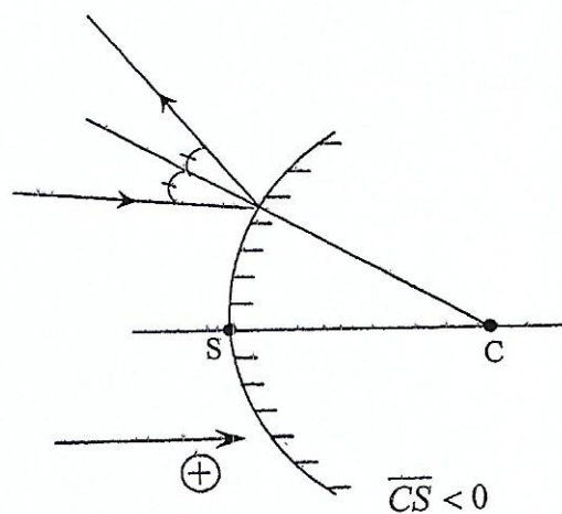
miroir convexe
