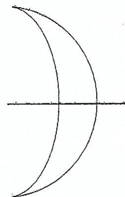
Ménisque convergent
