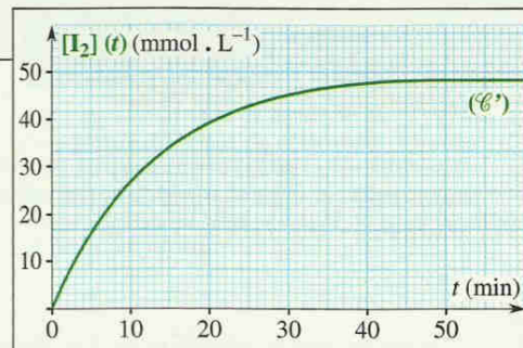
Doc. 7 Courbe [I_2] = f(t) .
