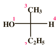
butan-2-ol "R"
