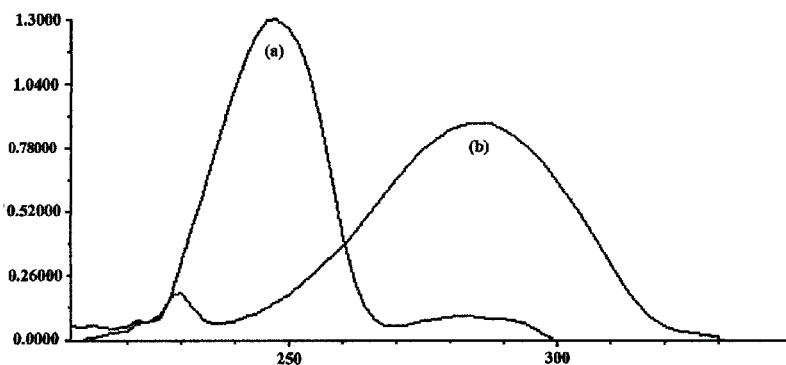
Figure 4.5 Exemples de spectres UV. (a) Benzaldéhyde (Ph-CHO), (b) Cinnamaldéhyde (Ph-CH=CH-CHO).
