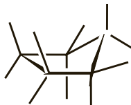
cyclopentane
