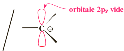
Figure 5.3 Structure du carbocation.
