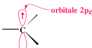
Figure 5.4 Structure du radical.
