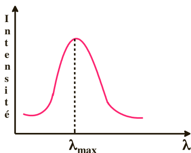
Figure 4.3 Spectre UV-visible typique.
