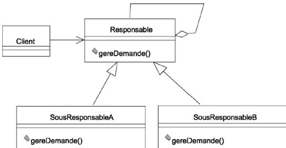
Figure 24–10 Le pattern Chain of responsibility
