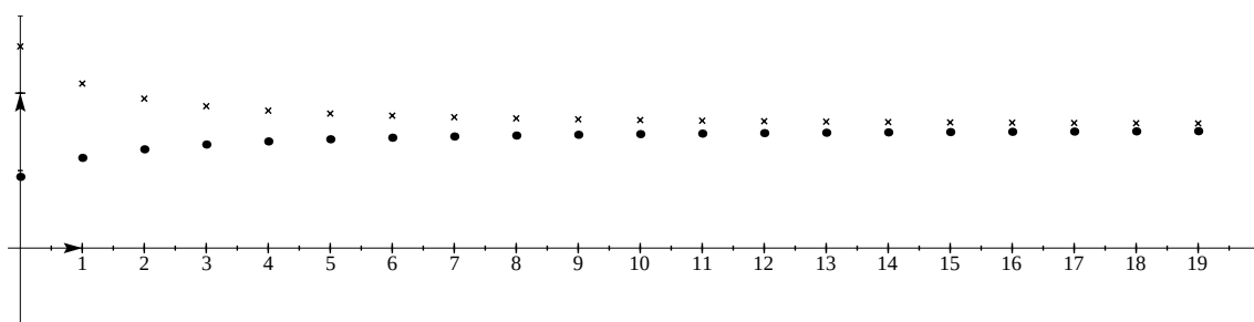
FIGURE 10.2 – Suites adjacentes
