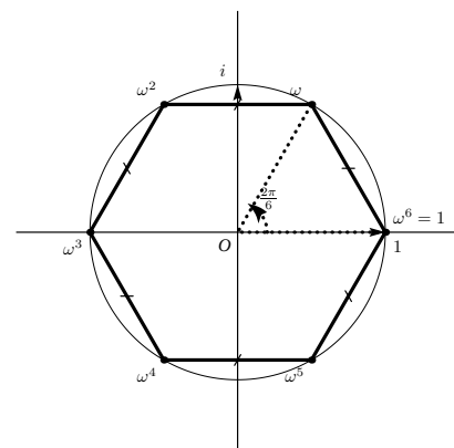
FIGURE 1.11 – \mathbb{U}_6
