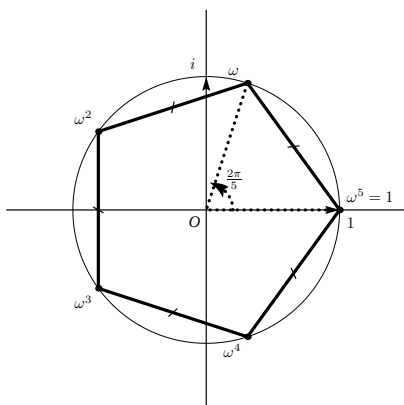
FIGURE 1.10 – \mathbb{U}_5
