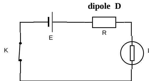
circuit b
