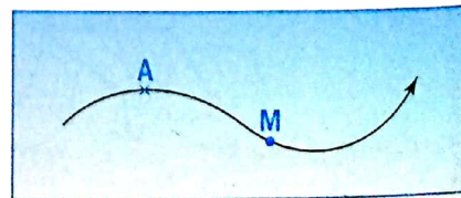
Fig. 4. Abscisse curviligne s = \widehat{AM}
