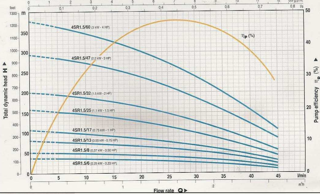
PERFORMANCE CHART AT n= 2900 1/min
